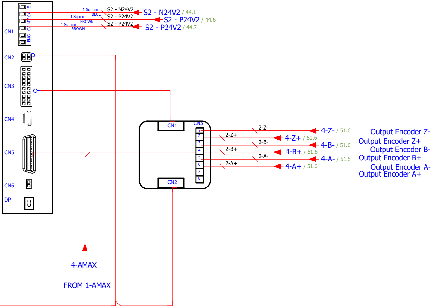
TAKE SPRING INTEGRATED SHAFT U2
